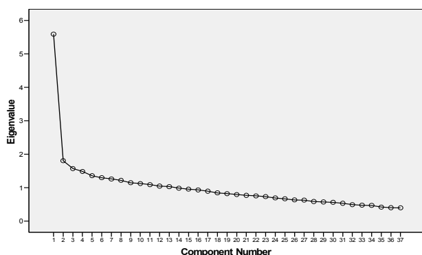
Scree Plot
